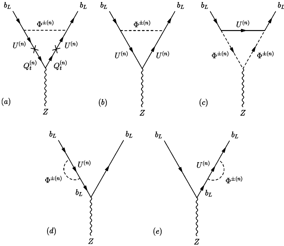
FIG. 3. Dominant UED contributions to the Zb\bar{b} vertex.
