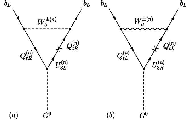
FIG. 4. Diagrams giving subleading contributions to the G^0 b \bar{b} vertex.
